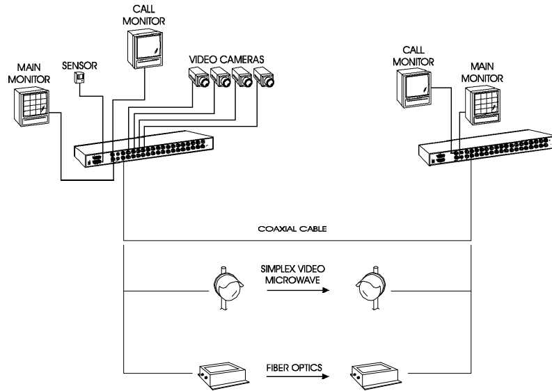
Figure 3 — One-Way Multiplexed Video Transmission
