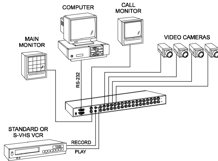
Figure 4 — MUX-1602C System with RS-232 Control
