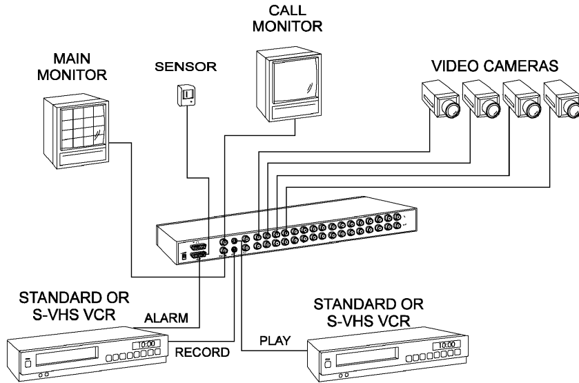
Figure 2 — MUX-1602C System with Two VCRs
