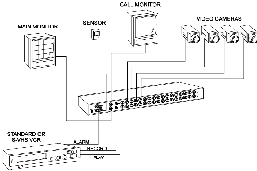
Figure 1 — Basic MUX-1602C System
