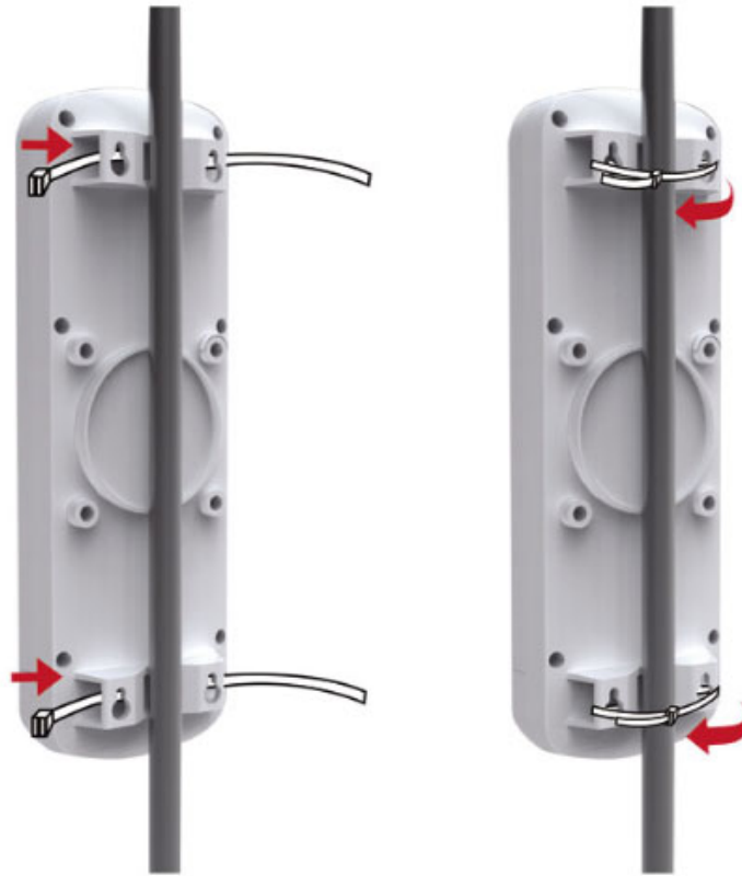
Figure 3-5 Pole Mounting
