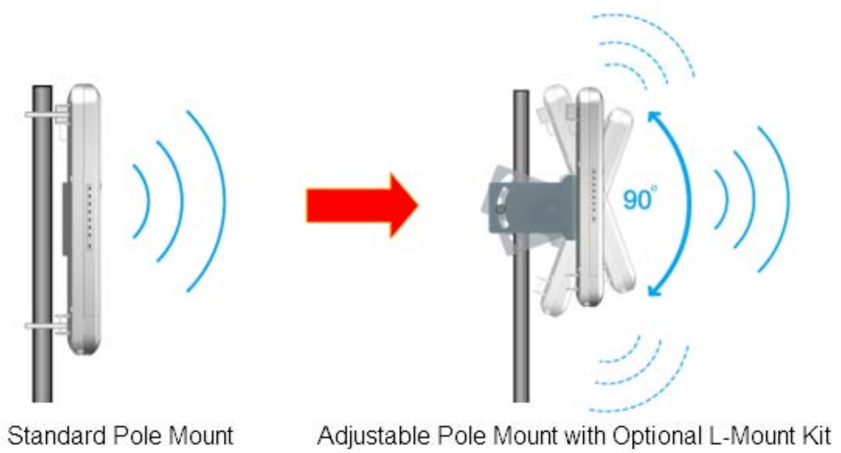
Figure 3-6 L-Mount – Adjustable antenna
