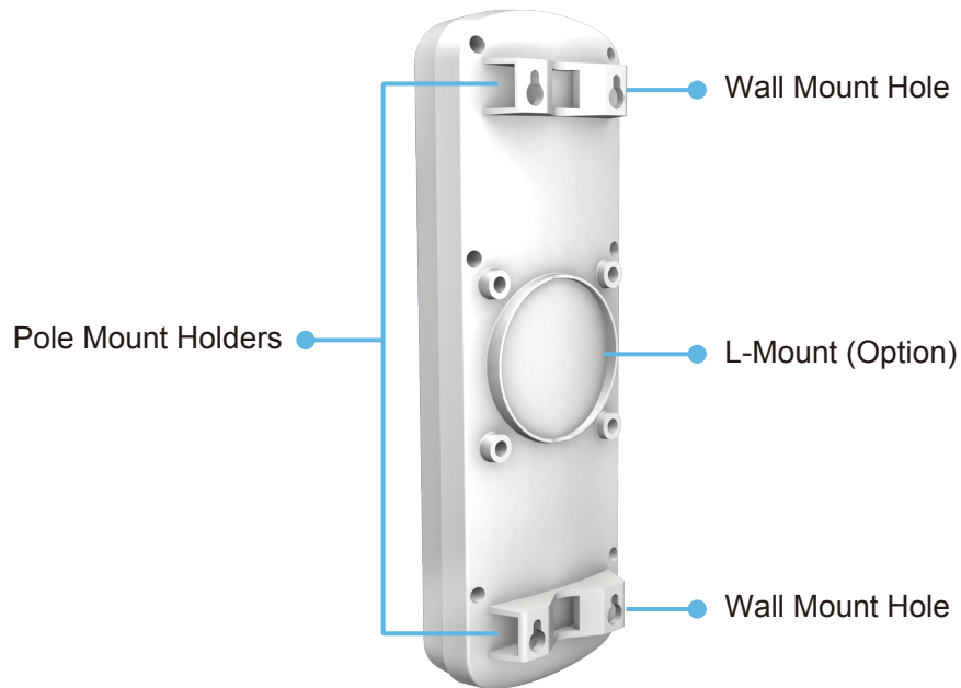
Figure 2-3 Mounting Design
