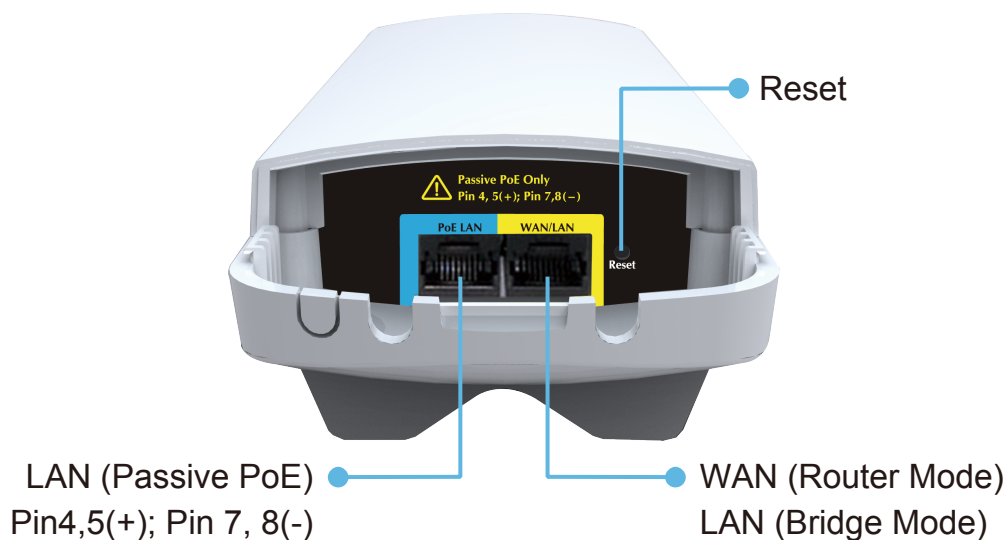
Figure 2-5 Bottom Panel
