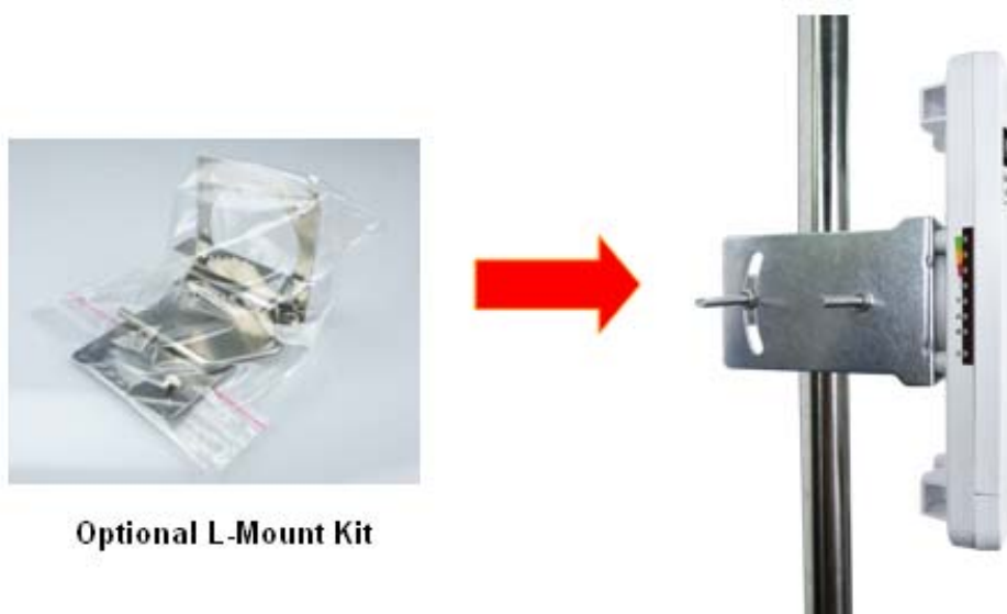
Figure 3-5 L-Mount
