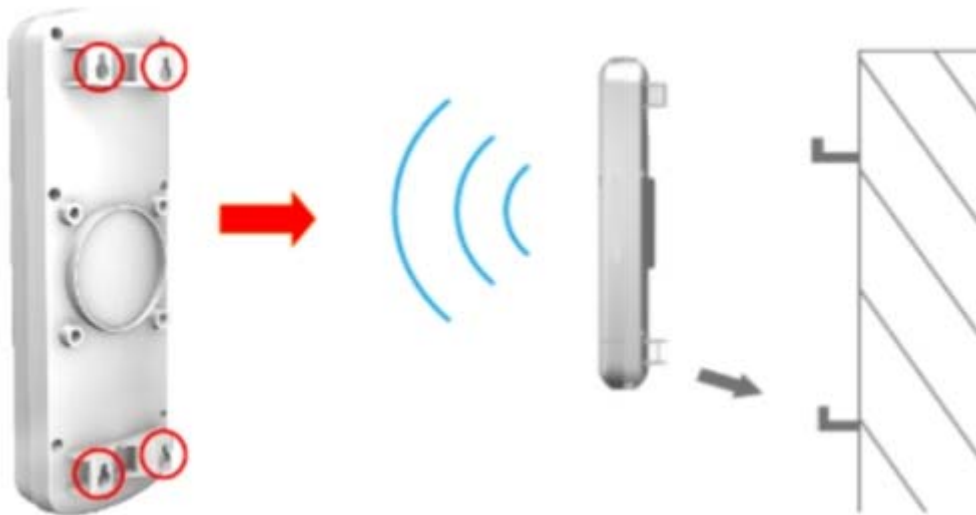
Figure 3-7 Wall Mount
