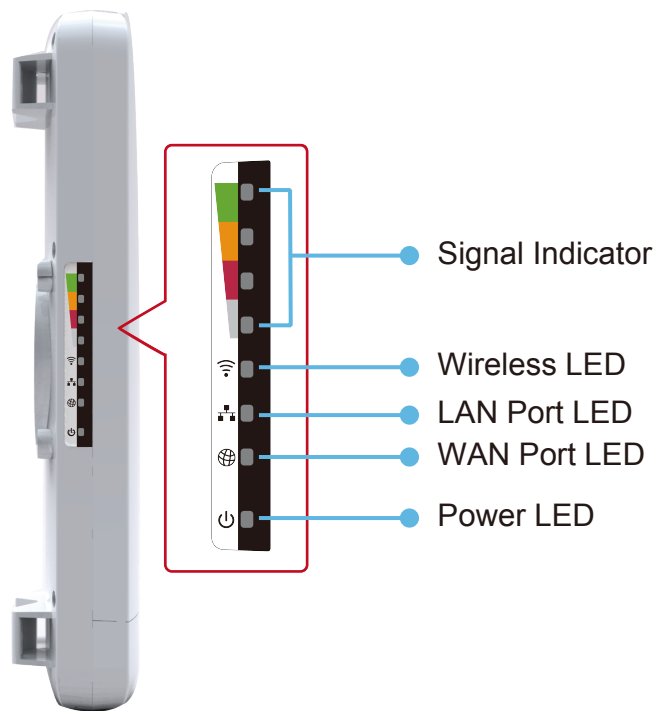
Figure 2-2 LED
