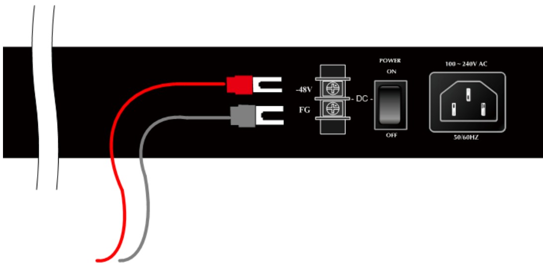
Figure 2-23 -48VDC connector
