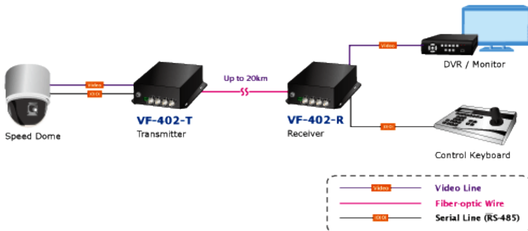
Figure 3-2 VF-402-T / VF-402-R stand alone installation
