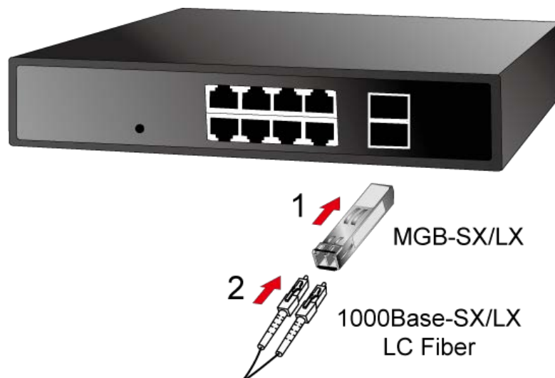
Figure 2-7 Plug in the SFP transceiver
