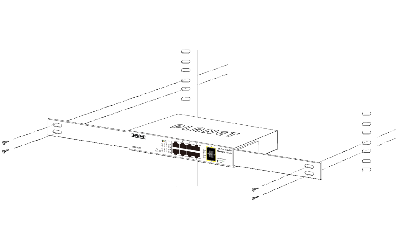
Figure 2-6 Mounting Managed Switch in a Rack
