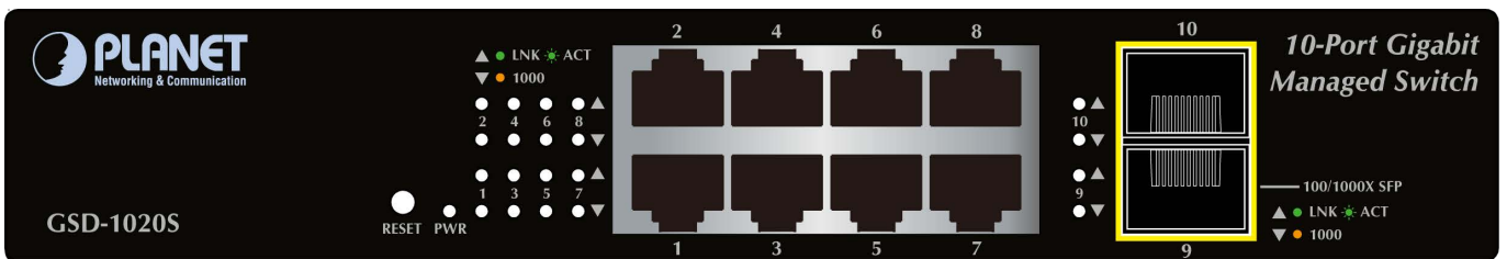
Figure 2-2 GSD-1020S LED panel
