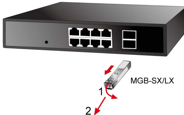
Figure 2-8 How to Pull Out the SFP Transceiver
