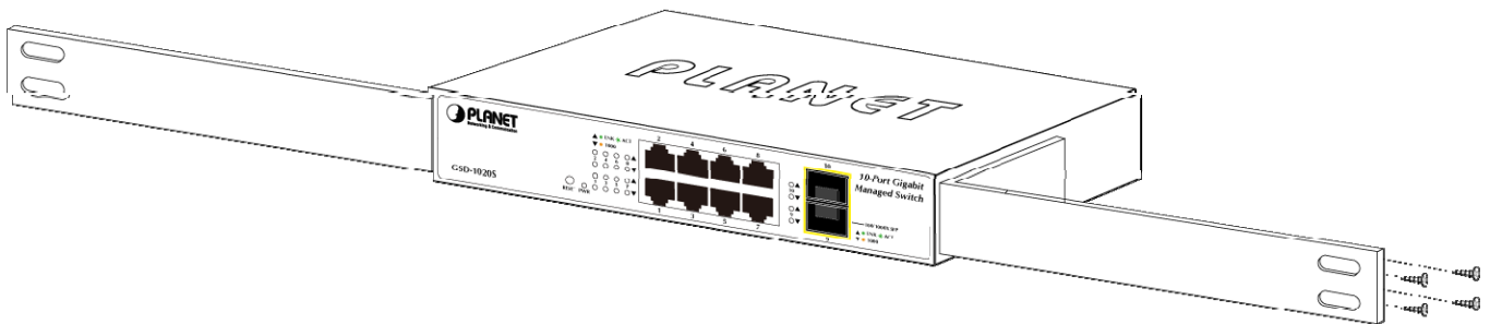
Figure 2-5 Attach Brackets to the Managed Switch.
