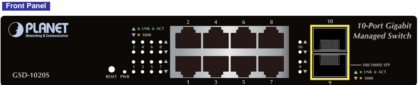
Figure 2-1 GSD-1020S front panel
