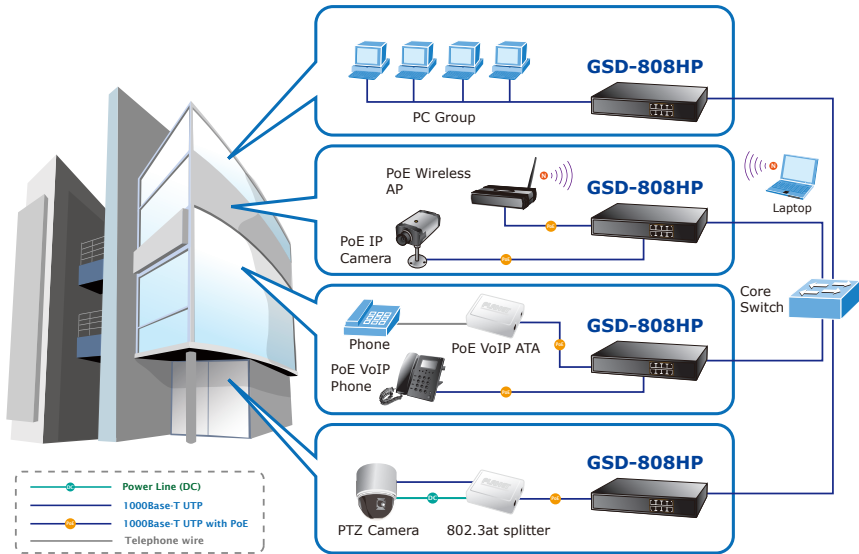
Figure 2-7: IP Office Department / Workgroup PoE Switch Connection
