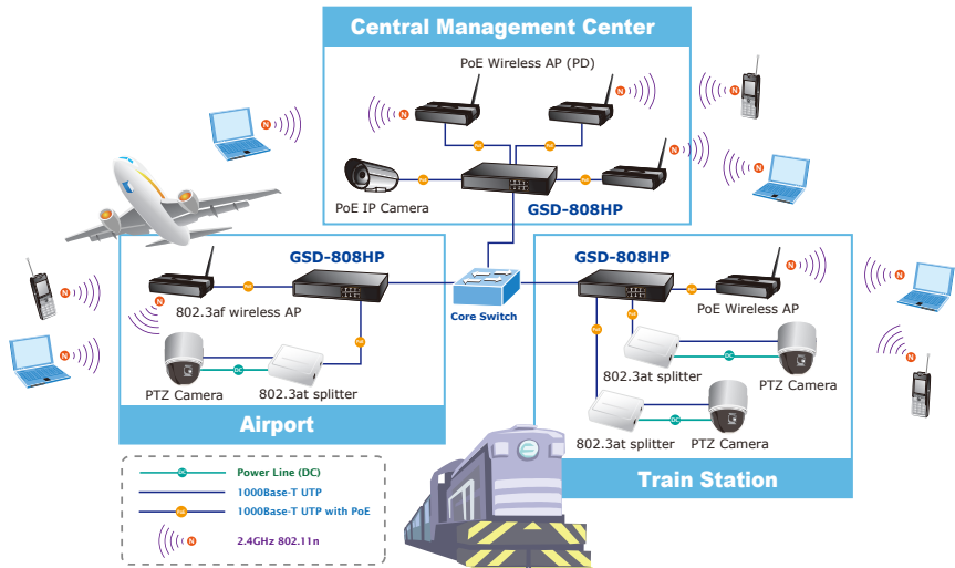
Figure 2-6: End Node or Switch Connection
